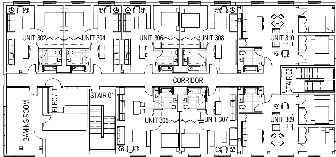
3 LEVEL 03 3/64" = 1'-0"
