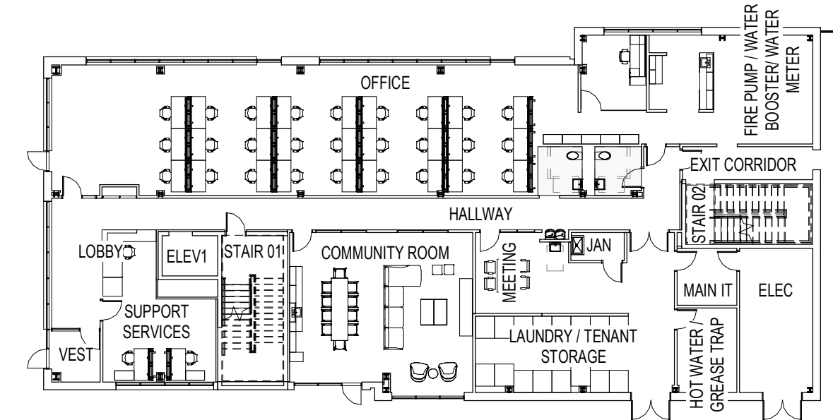
1 LEVEL 01 3/64" = 1'-0"
