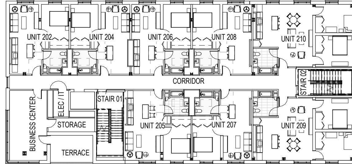
2 LEVEL 02 3/64" = 1'-0"
